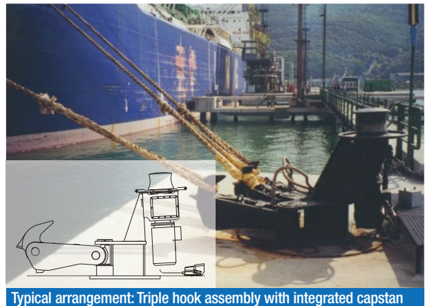
Typical arrangement: Triple hook assembly with integrated capstan
